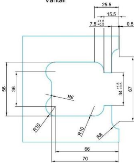
Türblatt Vantail
