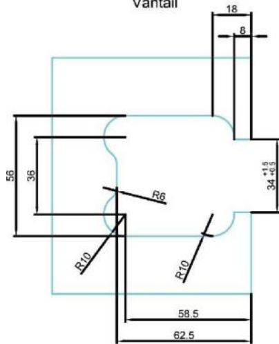
Türblatt Vantail
